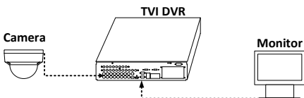
Figure 3-1 Connection
