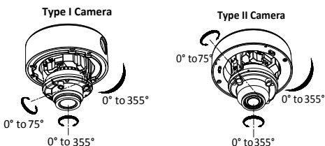
Figure 2-4 3-Axis Adjustment
