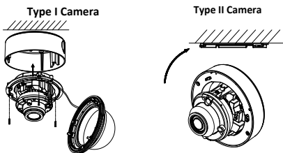
Figure 2-3 Fix the camera to the Ceiling
